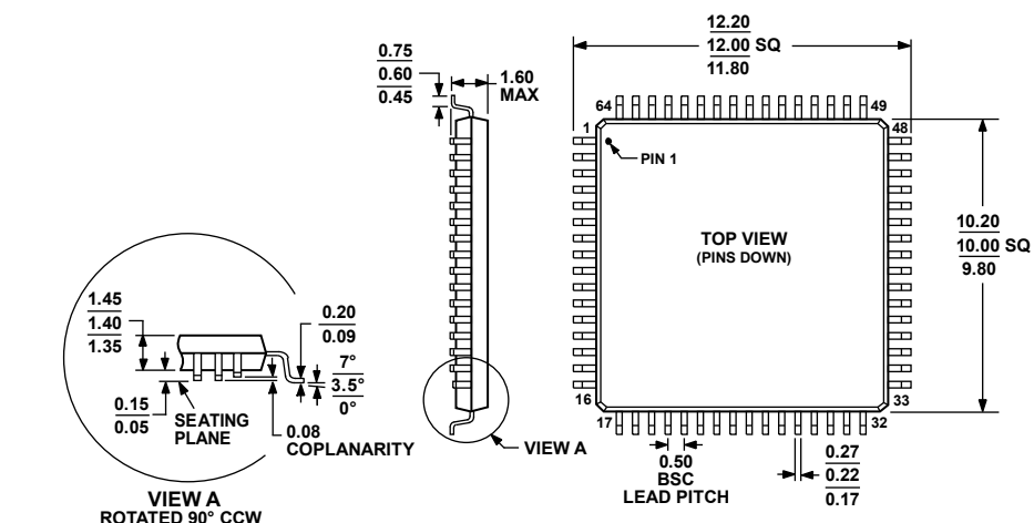
Figure 6. 64-Lead Low Profile Quad Flat Package [LQFP] (ST-64-2)
